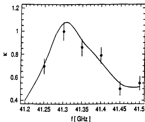
Fig. 4. Frequency dependence of EHF EMR effect on radiation-induced repair of the genome conformational state of E. coli AB1157 cells (20 Gy; 200 \mu W/cm 2 , 10 min).
