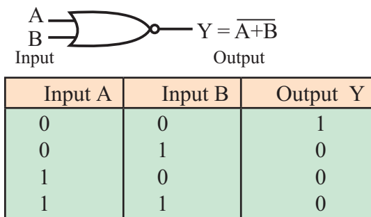
Fig. 16.31: NOR gate symbol and its Truth table.
