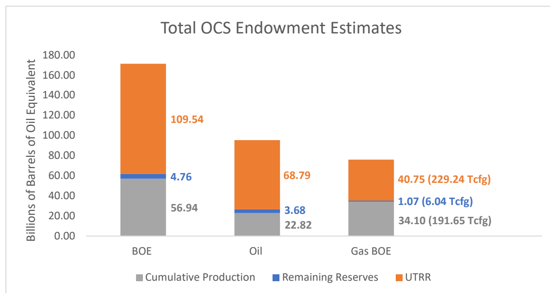
Figure 9. Distribution of total hydrocarbon endowment by type and resource category. Gas values are represented in BOE for comparative purposes. Values for cumulative production and reserves are based on data available as of January 1, 2019.
