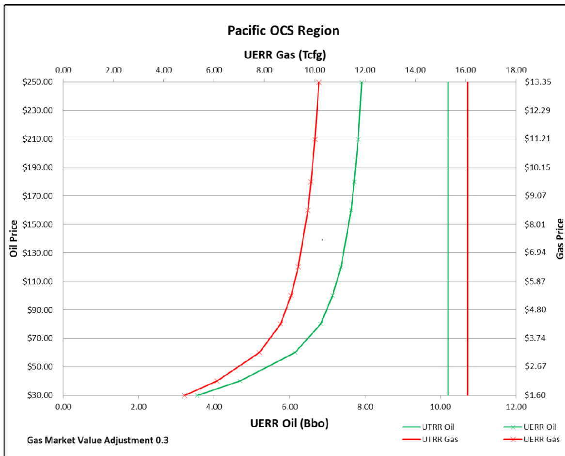
Figure 28. Price-supply curve for the Pacific OCS region.
