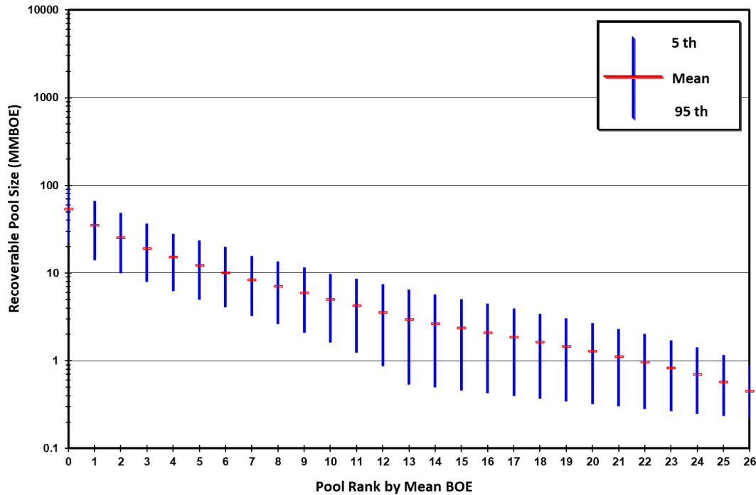
Figure 6. Sample lognormal field size distribution ranked by mean pool size.
