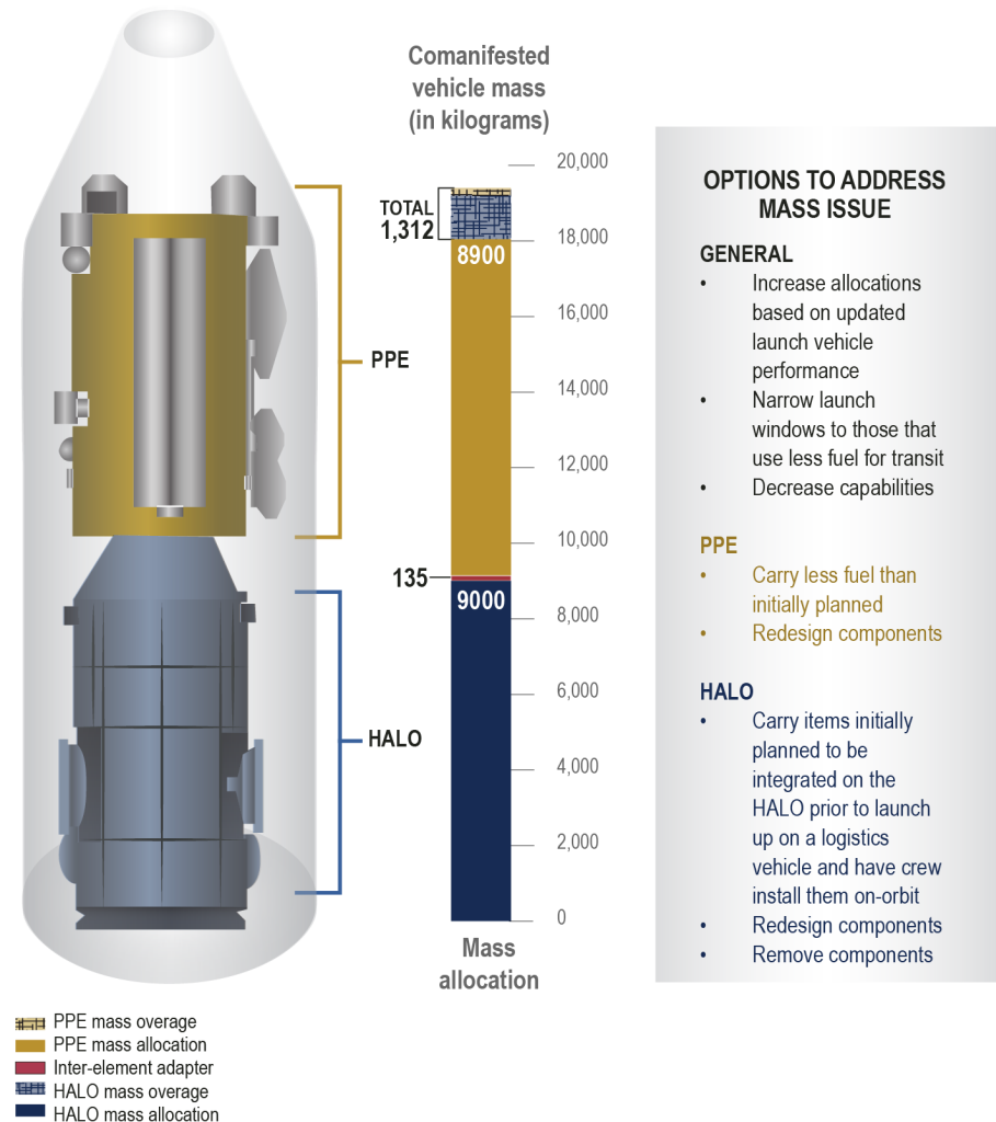
Figure 6: Comanifested Vehicle Mass and Options to Address Habitation and Logistics Outpost (HALO) and Power and Propulsion Element (PPE) Mass Growth Over Allocations
