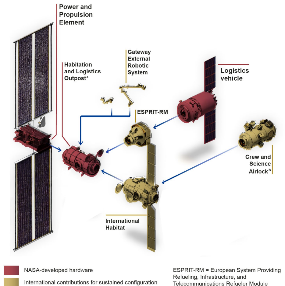
Figure 1: Illustration of the Gateway Sustained Configuration
