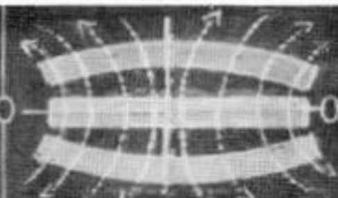
Fig. 165. LENSES WHICH CURVE OUTWARD FROM EQUATORS.
