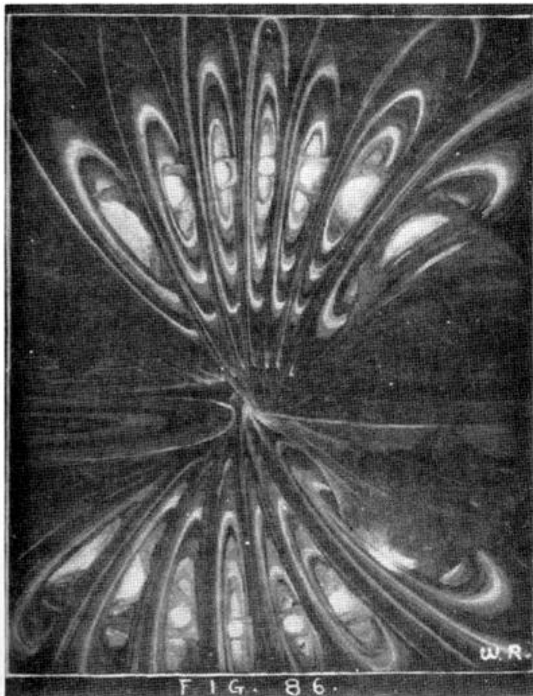
FIG. 86. CROSS SECTION OF OCTAVE WAVE ILLUSTRATING THE GYROSCOPIC SPIRAL PRINCIPLE OF MULTIPLICATION OF POWER BY ACCELERATING SPEED CENTRIPETALLY TO BUILD A SPHERE, THEN DIVIDING POWER BY DECELERATING SPEED CENTRIFUGALLY UNTIL MOTION IS AGAIN ZERO AT WAVE AXIS.
