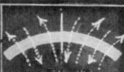
Fig. 163. LIGHT PRESSURES CREATE LENSES TO BEND LIGHT.
