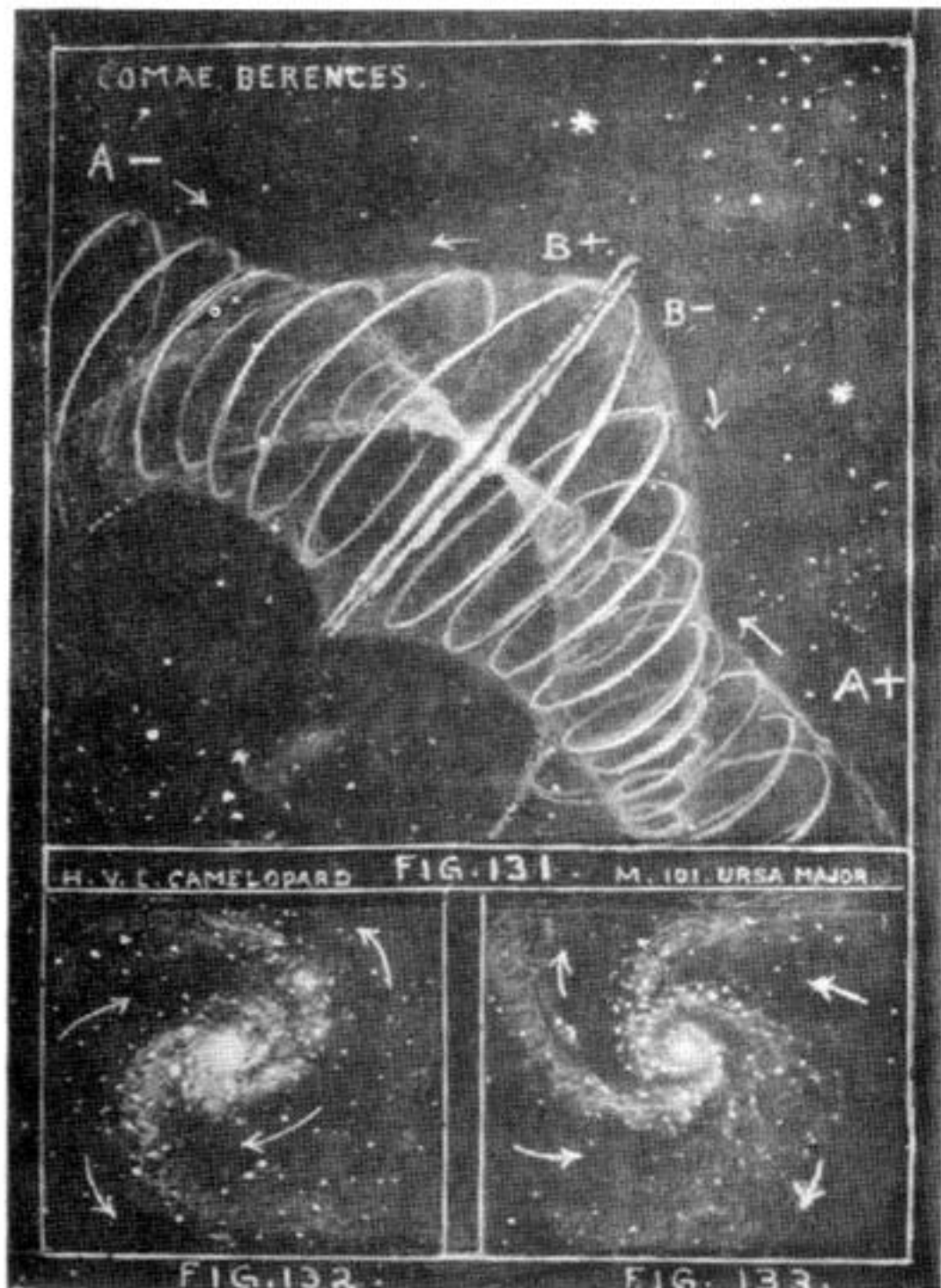
Fig. 131 ILLUSTRATES METHOD OF CREATING INCANDESCENCE BY MULTIPLYING DARKNESS, INCANDESCENCE IS THEN DIVIDED TO AGAIN BECOME DARKNESS, Figs. 132 and 133 SHOW GIANT NEBULAE COMPRESSING DARKNESS INTO LIGHT, AND EXPANDING LIGHT INTO DARKNESS TO CREATE BODIES AND DESTROY THEM.
