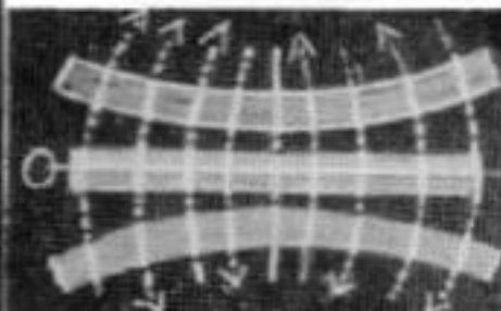
Fig. 164. LENSES WHICH CURVE INWARD TOWARD EQUATORS.
