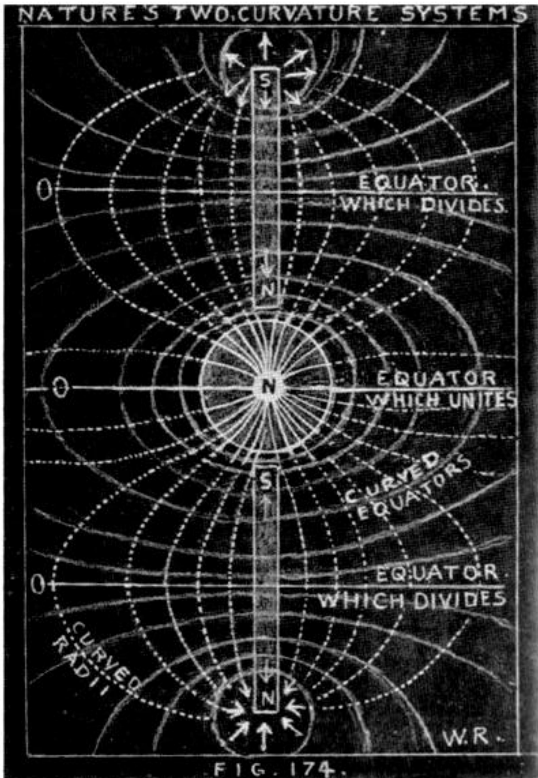
ILLUSTRATING NATURE'S REPRODUCTIVE PROCESS. CURVATURE FOR DIVIDED PAIRS MUST REVERSE FOR UNITED PAIRS. TWO EQUATORS MUST BECOME ONE AND TWO CENTERS OF GRAVITY MUST ALSO BE ONE.
