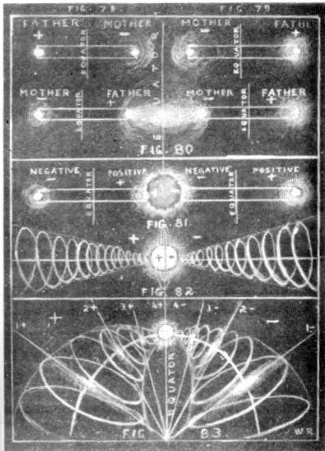
ILLUSTRATING THE FATHER-MOTHER PRINCIPLE OF BUILDING BODIES BY DIVIDING LIGHT INTO POLARIZED UNITS - AND REPRODUCING BODIES BY UNITING TWO WAVE-FIELDS OF OPPOSED UNITS INTO ONE.
