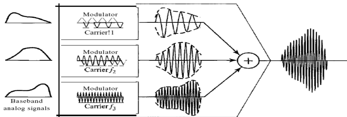
Figure 2 FDM process
