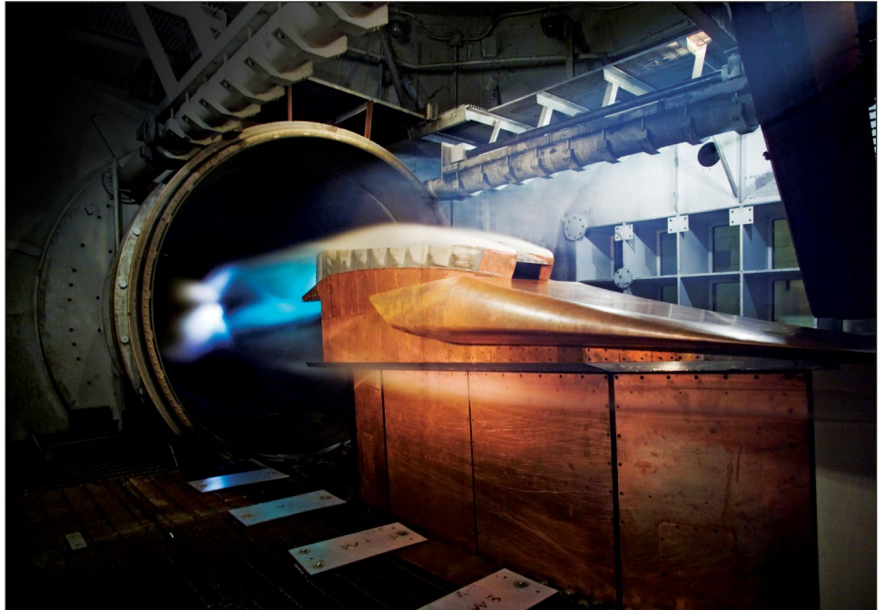
Figure 5: NASA Langley's Hypersonic Model Test in the 8-Foot High Temperature Tunnel
