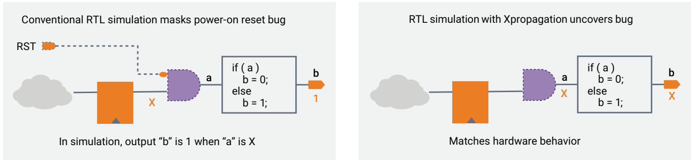
Figure 9: VCS Xpropagation support
